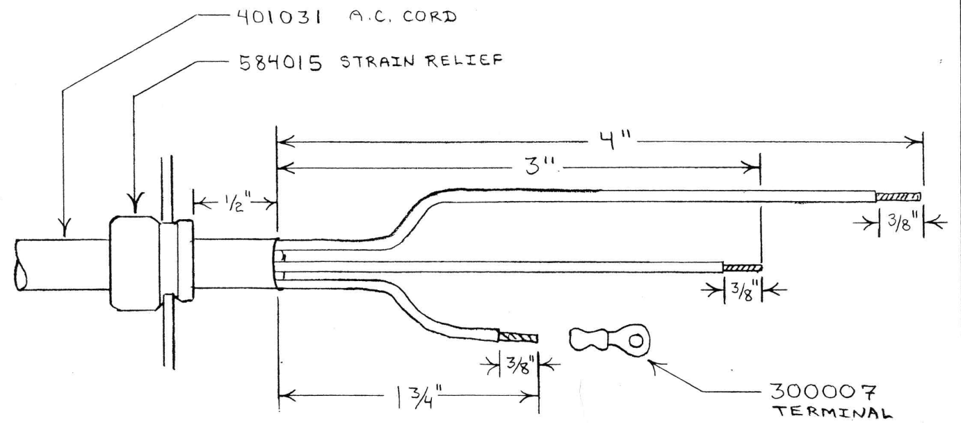
POWER CORD STRIPPING DETAILS
