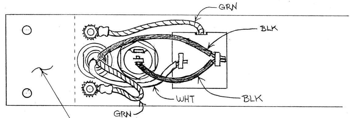
KEEP THIS AREA CLEAR REAR PANEL WIRING DETAILS
